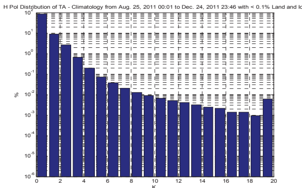
Figure 3: (large top) Peak hold RFI map of the largest deviation of brightness temperature from the average RFI-free value over the period 25 Aug – 24 Dec 2011 highlights the regions of prevalent RFI over the ocean. (small bottom) Histogram of the samples in Fig. 3-top. The largest (20 K bin) accounts for all samples at or above 20 K.
